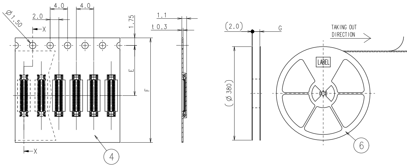
CARRIER TAPE (S=2/1)
