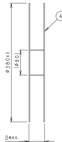
SECT. E-E
