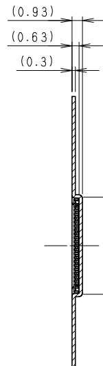
SECT. E-E
