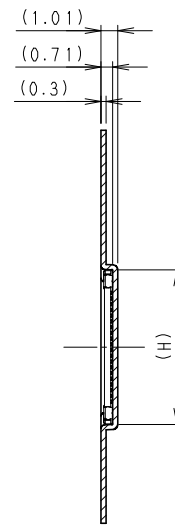
SECT. E-E
