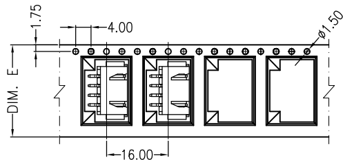
02~04 CONTACTS
