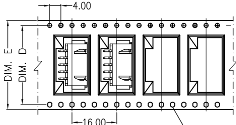
05~14 CONTACTS
